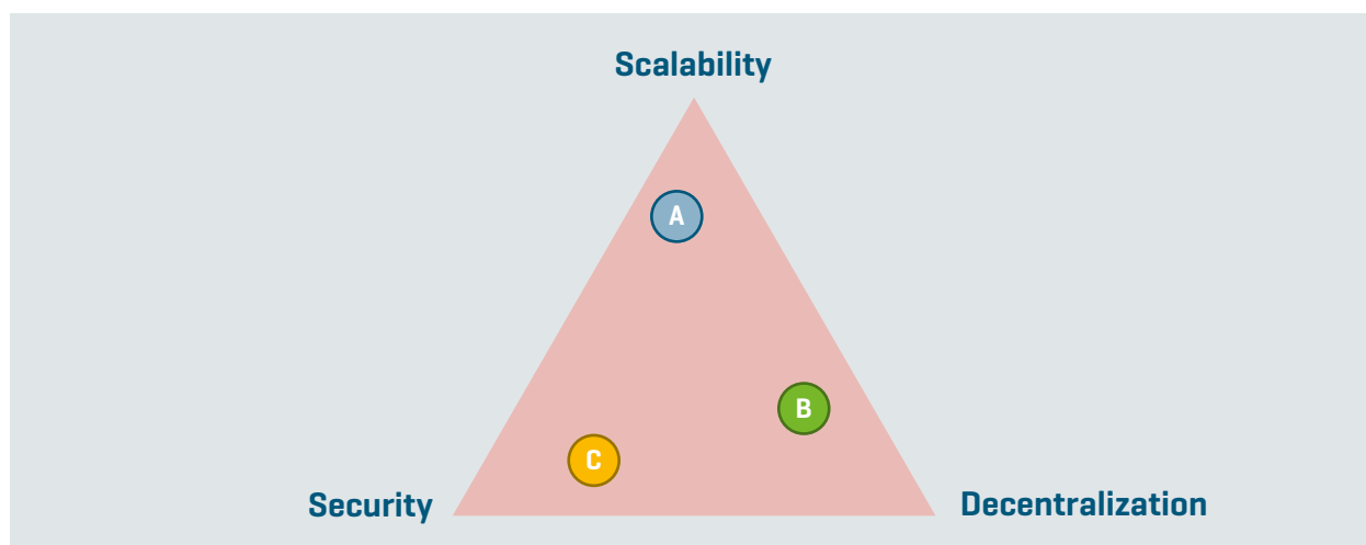
Figure 11: The distributed ledger trilemma. Blockchain designs A, B and C cannot enjoy all three ideal properties fully and simultaneously
